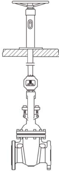
Floor stand
